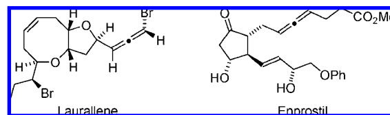
Figure 1. Naturally occurring and biologically active allenenes.
